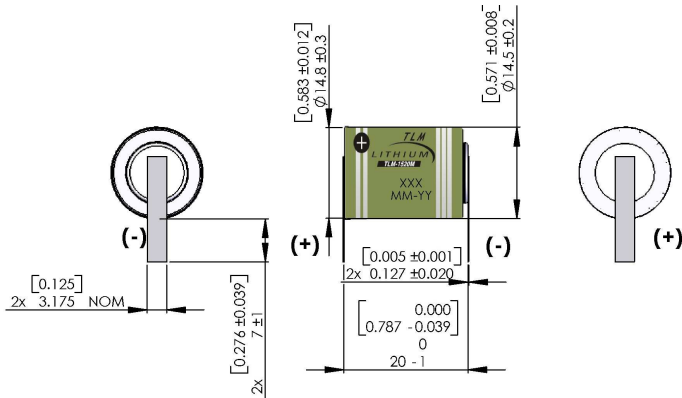
TLM-1520M/T (Soldering Tabs) Cat. # 72142622150
